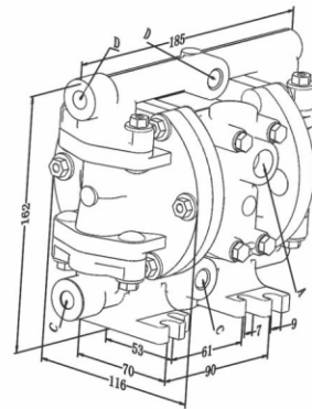
Polypropylene pump
